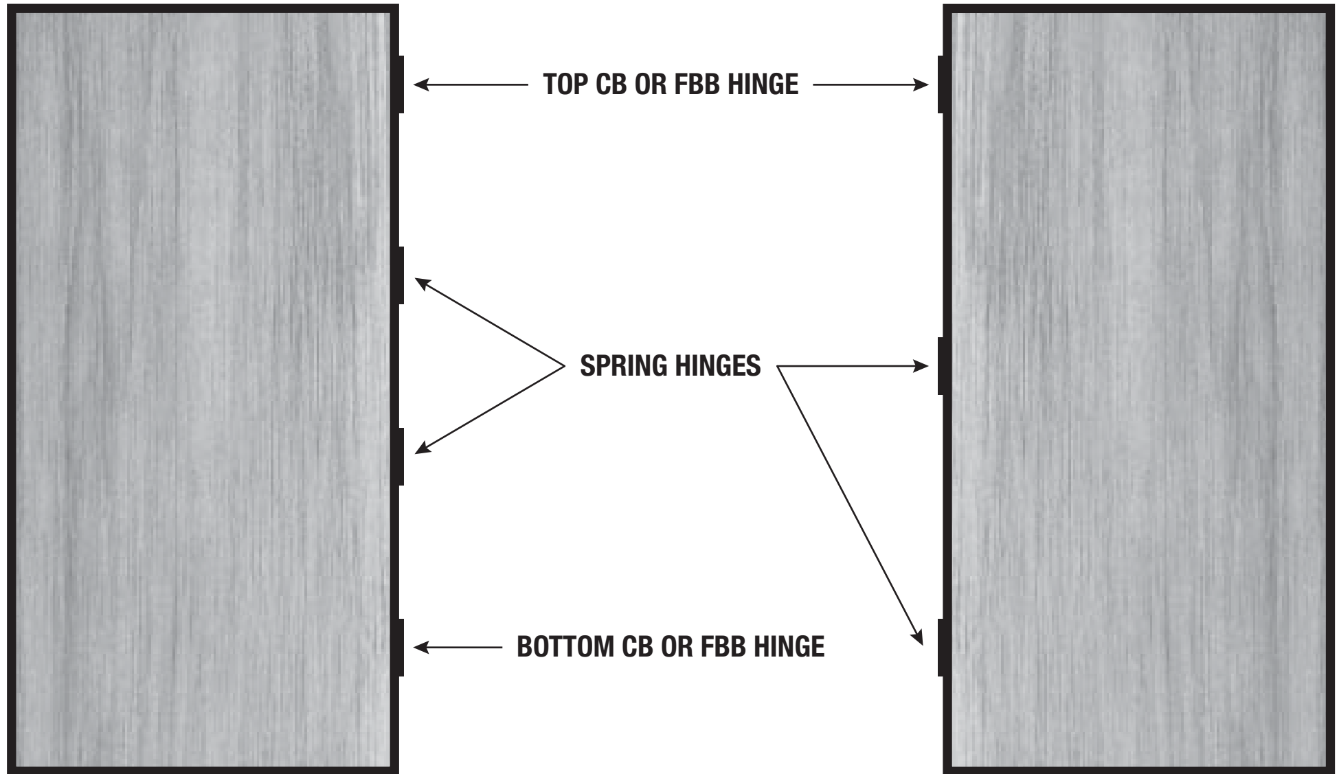
TYPICAL DOOR ELEVATION WHEN USING 3 HINGES
